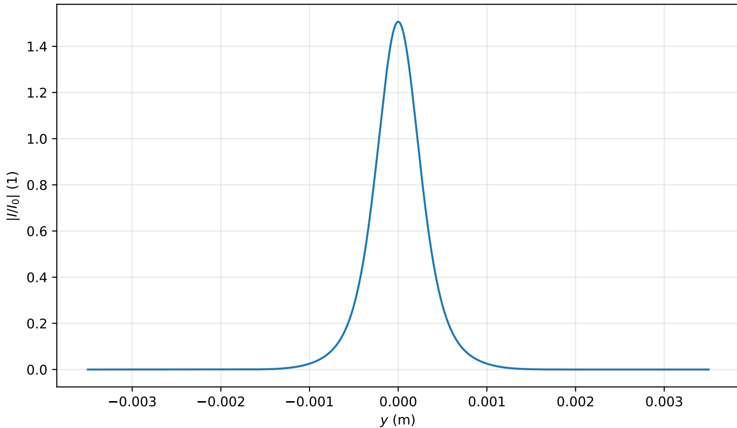
Intensity profile I(x=0, y, z=1.274)/I_0 , P_{in}=0.9P_{cr} , artificial time
